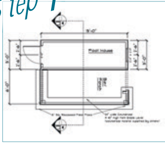
2-D Drawing
